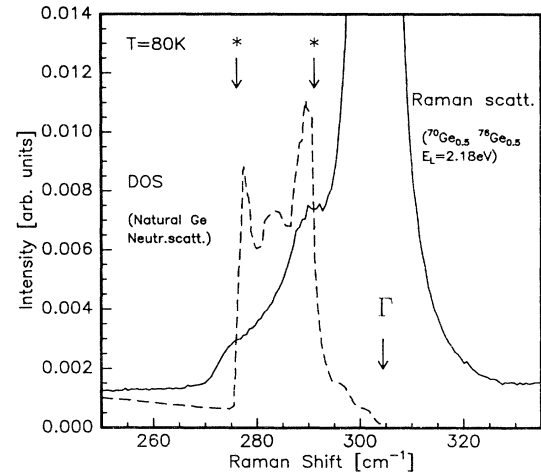
FIG. 2. Raman spectra of ^{70}\text{Ge}_{0.5}^{76}\text{Ge}_{0.5} (solid line) compared to the phonon density of states (DOS, dashed line) at 80 K. The Raman spectra were taken with the 568.2\text{ nm} line of an \text{Ar}^+ laser. The dominant band modes (marked with * ) appear at the edges of the DOS. The scattering intensities are normalized so that the peak of the Raman-active mode at \Gamma (off scale) is equal to 1.
