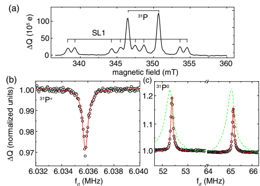
FIG. 2 (color online). (a) EDMR spectroscopy of the ^{31}\text{P} and SL1 electron spin transitions. Four additional field peaks related to the SL1 are observed outside the magnetic field range shown here. (b), (c) Spectroscopy of the nuclear spin transitions of the ionized ^{31}\text{P}^+ and the neutral ^{31}\text{P}^0 (open circles). Resonance frequencies and peak widths are extracted from Lorentzian fits (red lines). For comparison, the spectroscopy of ^{31}\text{P}^0 nuclear spins near the Si/SiO 2 interface is shown as well (dashed green line, data taken from [27]).
